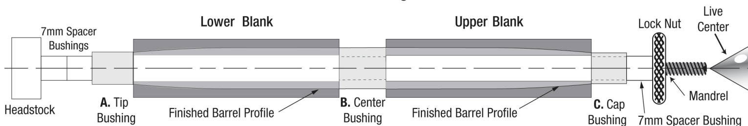
DIAGRAM B • Turning The Blanks
